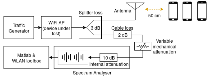
Fig. 1. The general setup used for all experiments. The total conducted pathloss consist of splitter loss (3 dB), cable loss (2 dB), variable mechanical attenuation (20 through 50 dB) and the internal attenuation of the spectrum analyser (10 dB).
